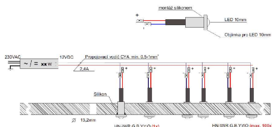
Schéma instalace - HN- x 10(R,G,B,Y) SET xx ks
